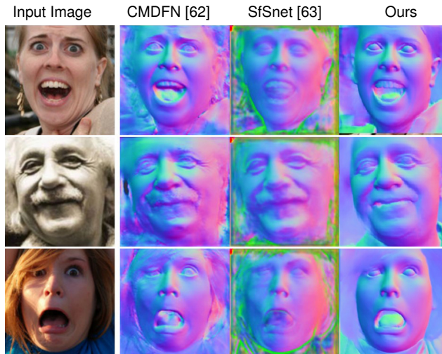
Figure 12: Qualitative Comparison against SOTA. Our synthetic data-only U-Net yields predictions comparable to SOTA while being less noisy and more robust to lighting.
