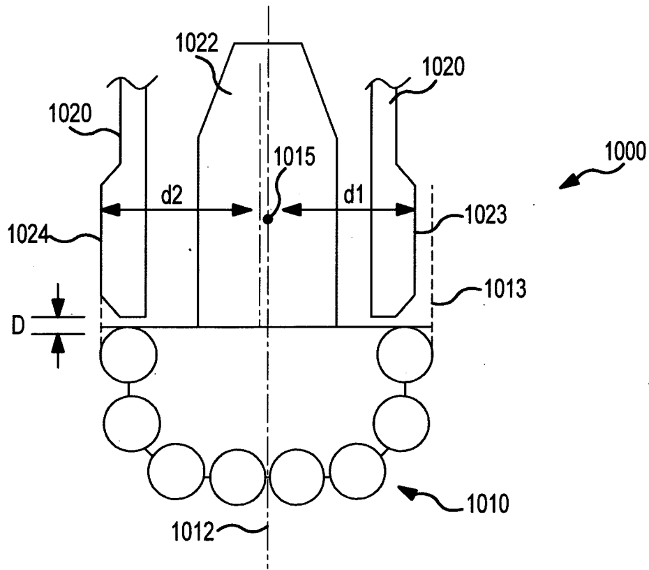
GAUGE PAD ASSEMBLY WITH CUTTER PROFILE.
